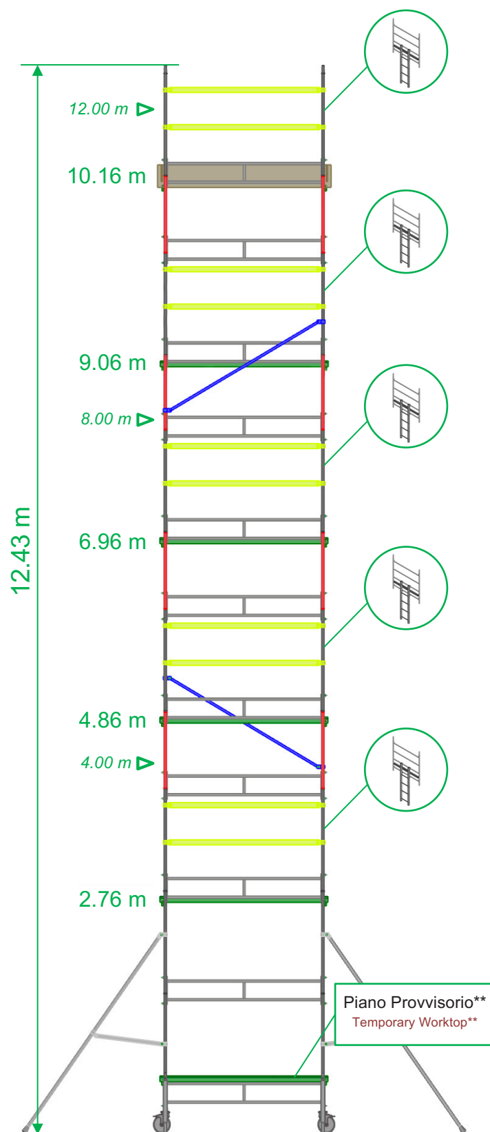
Mod. A+B+4C+D4+E: T124SP
