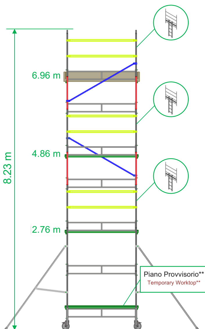
Mod. A+B+2C+D4+E: T082SP
