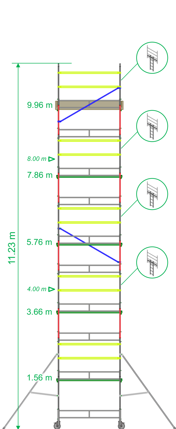
Mod. A+B+4C+E: T112SP
