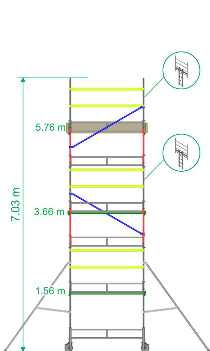
Mod. A+B+2C+E: T070SP
